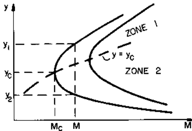
Figure 2-4. Typical Specific Force plus Momentum Curve (Barfield et al., 1981)
